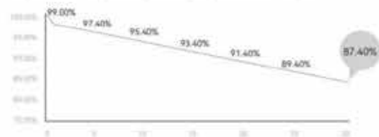
1st year -1%, 0.4% power degradation per year from 2 to 30 years
